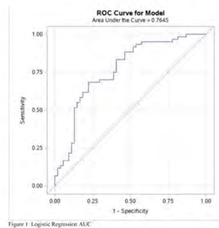
Figure 1: Logistic Regression AUC
