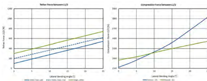
Fig. 1: Representation of the tether and intervertebral compression force between L1/2 for an 25° lateral bending task to the untethered side
